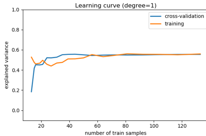
Fig. 20.5: For a degree=1 model
