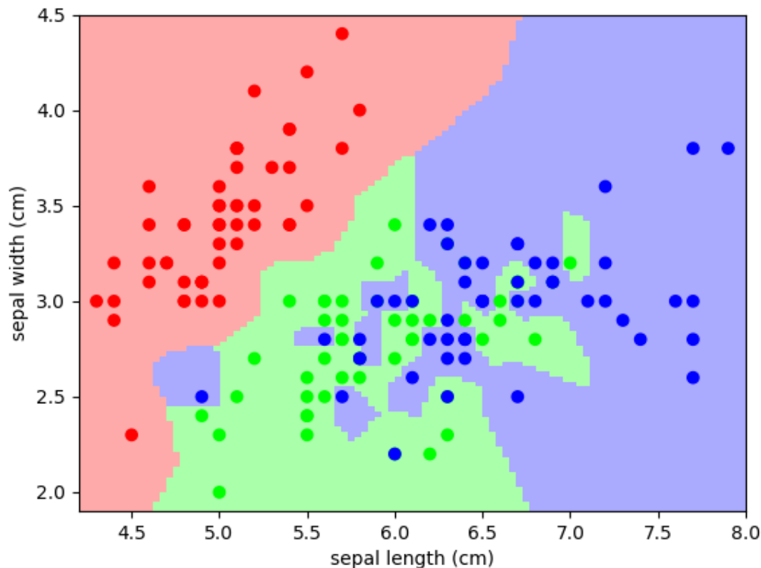
Fig. 20.3: A plot of the sepal space and the prediction of the KNN
