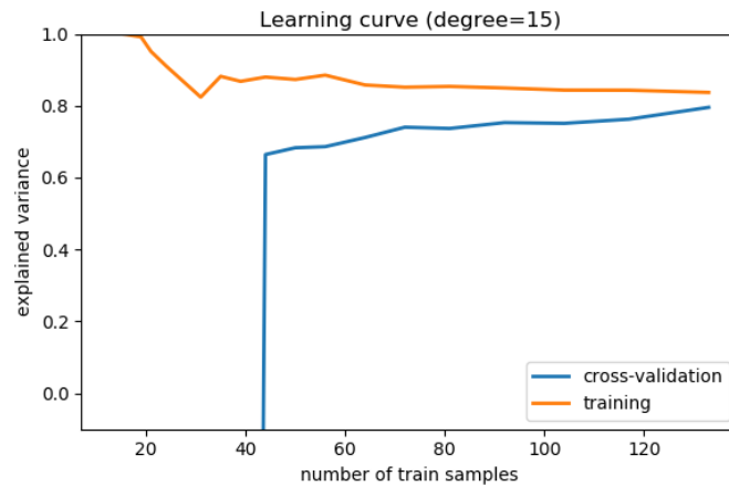
Fig. 20.6: For a degree=15 model
